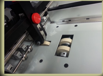
Bottom Friction Feed Rollers
